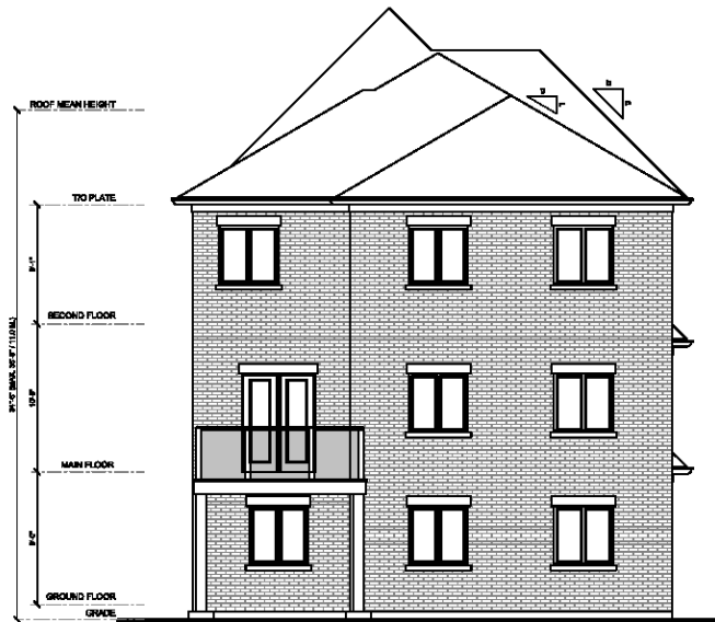
REAR ELEVATION - LOT 1
