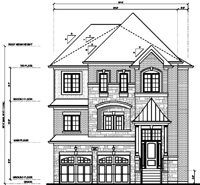
FRONT ELEVATION - LOT 1
