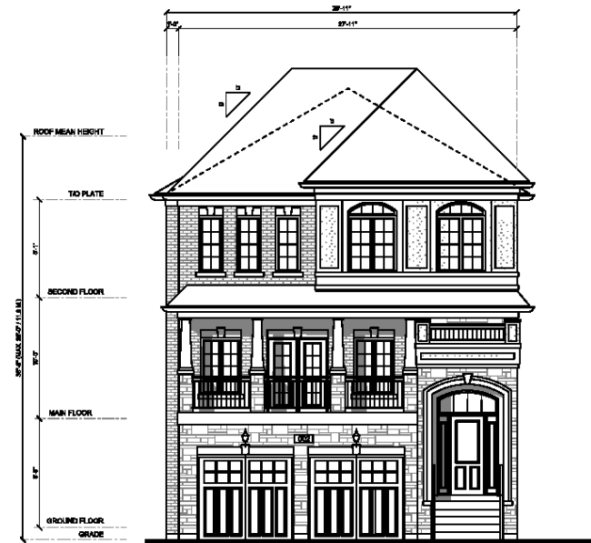
FRONT ELEVATION - LOT 2
