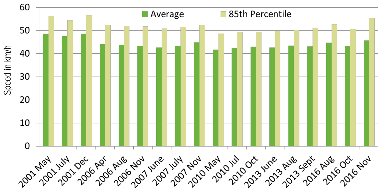
Figure 4: Historical Traffic Volume and Speed Observations on Hunter's Point Drive
