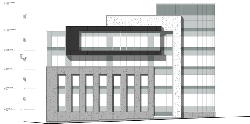
1 EAST ELEVATION A.3.1 1:150
