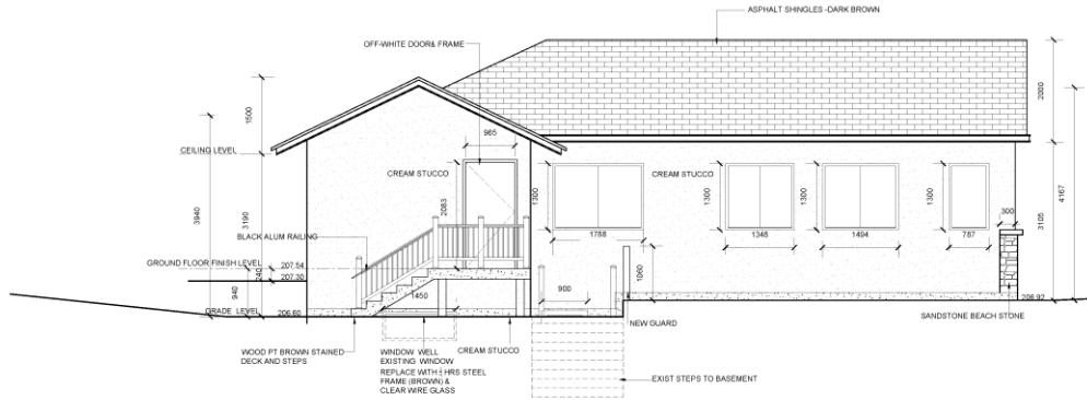
1 SOUTH ELEVATION - MAIN BUILDING & GARAGE SCALE 1 : 50 (1:100 17x11paper)
