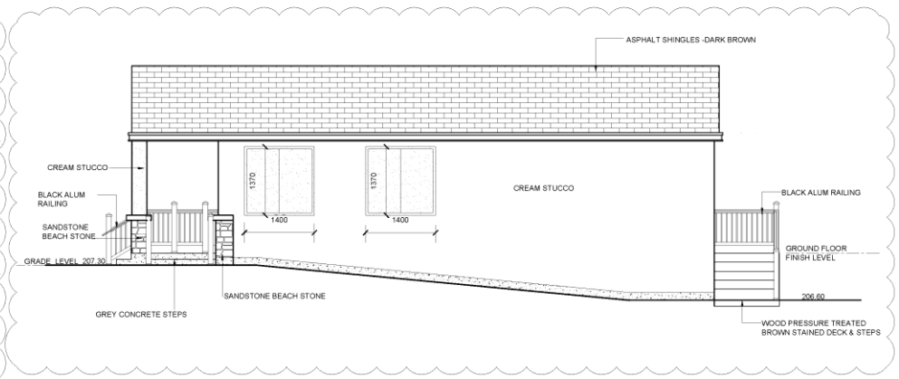
2 WEST ELEVATION - MAIN BUILDING SCALE 1 : 50 (1:100 17x11paper)
