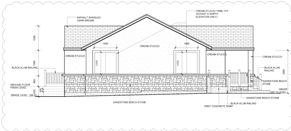
1 EAST ELEVATION - MAIN BUILDING SCALE 1 : 50 (1:100 17x11paper)
