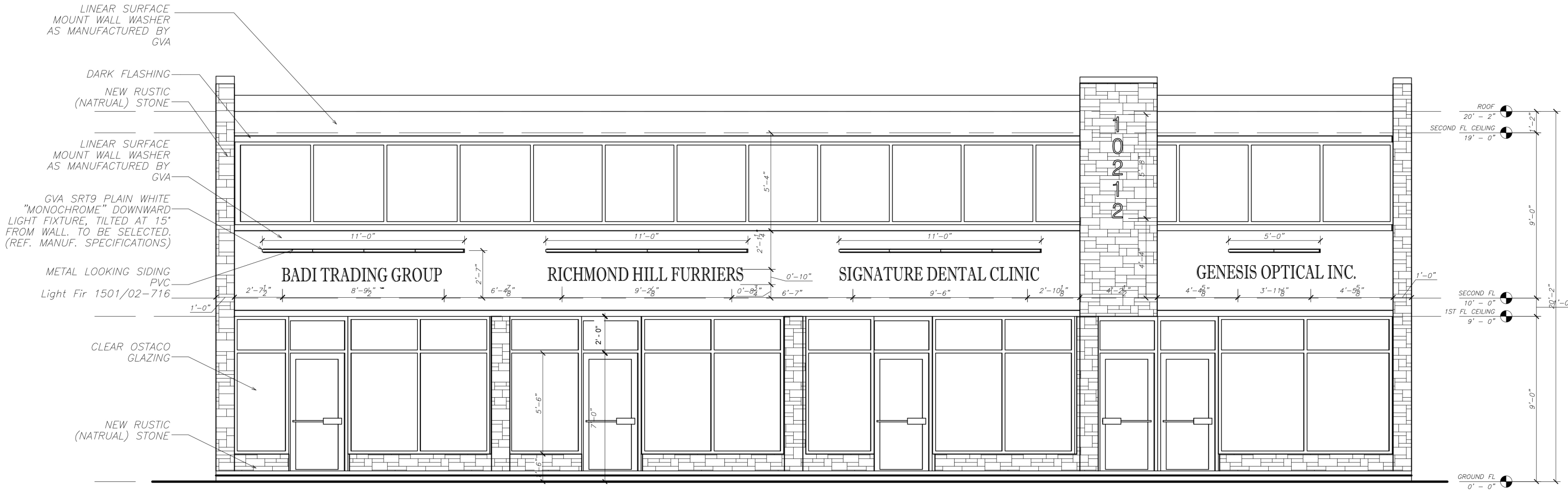
WEST ELEVATION
