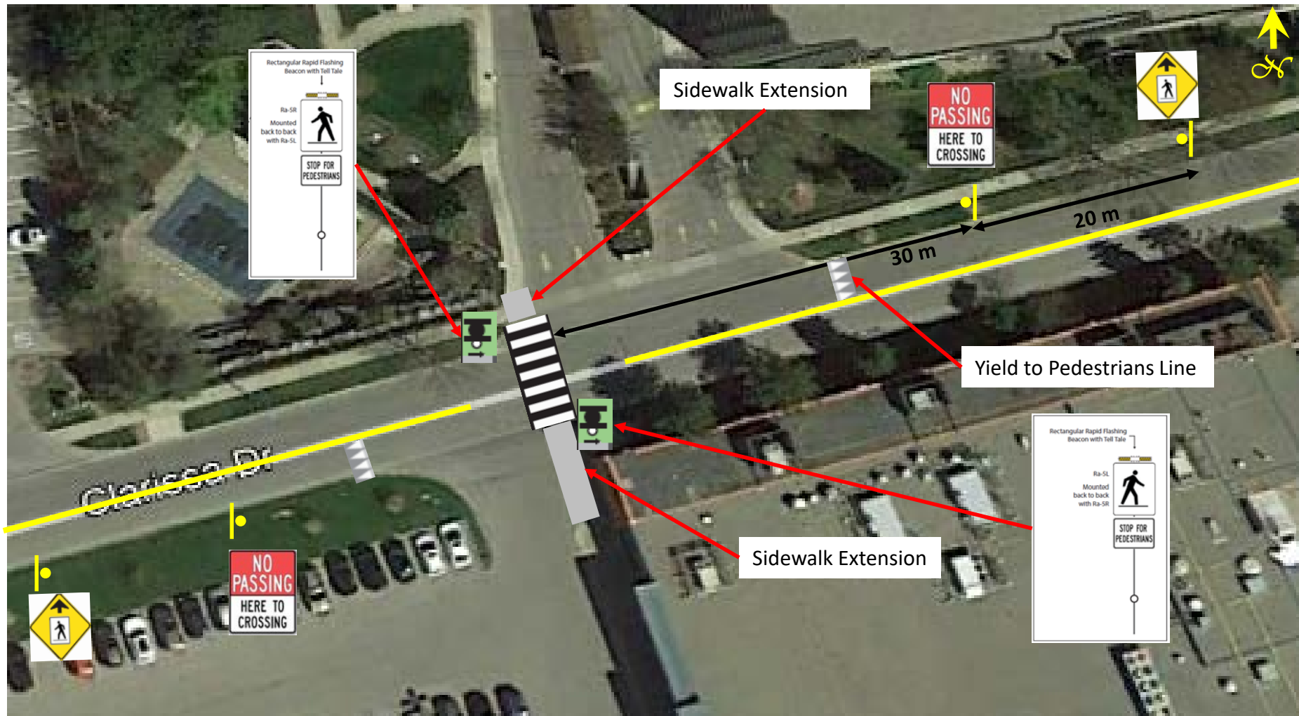
Figure: Pedestrian Crossing Improvements at Clarissa Drive
