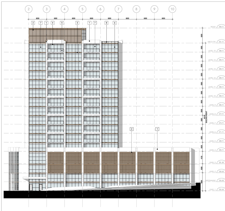
EAST ELEVATION SCALE: 1:200 2/44/07
