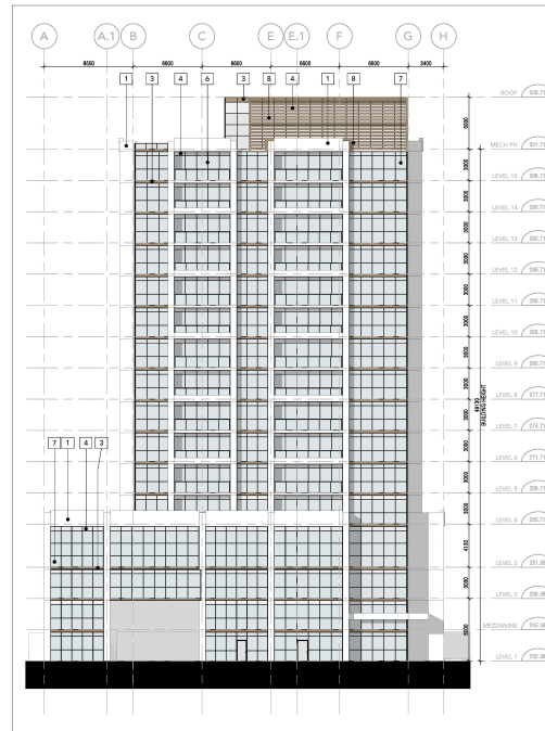
SOUTH ELEVATION SCALE: 1:200 1/44/07
