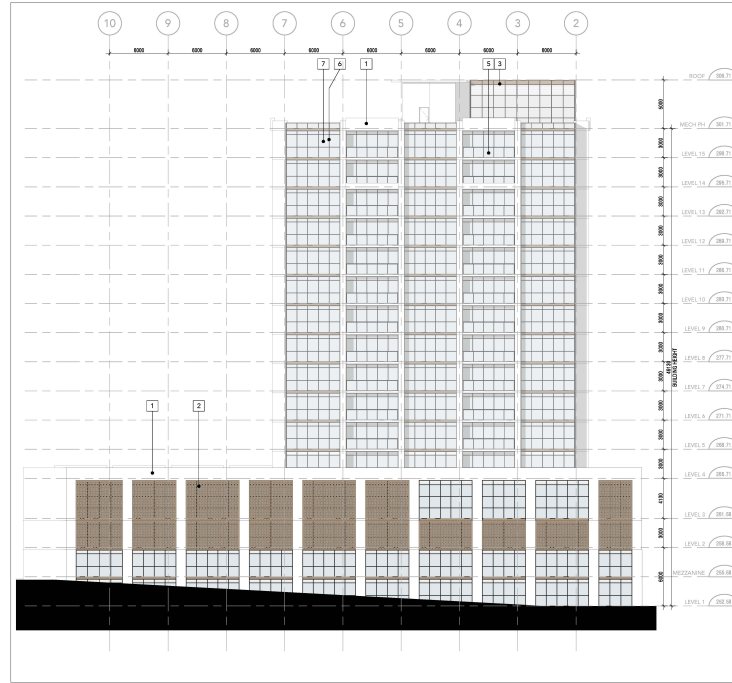
WEST ELEVATION SCALE: 1:200 1/44/07
