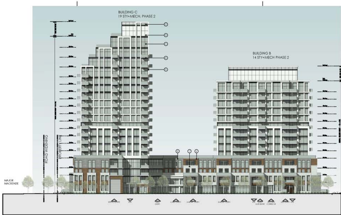
BUILDING B AND C EAST ELEVATION
