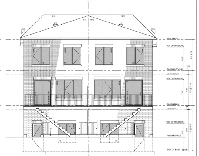
PROPOSED REAR ELEVATION SCALE AS NOTED OTHERWISE (UNIT 2) PROPOSED FRONT ELEVATION SCALE AS NOTED OTHERWISE (UNIT 1)
