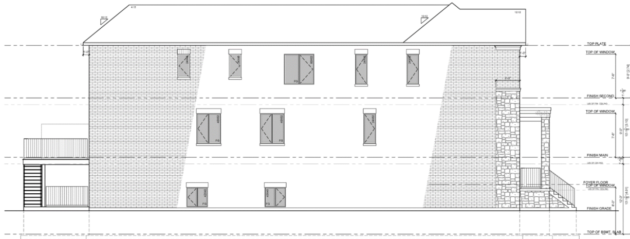
PROPOSED RIGHT SIDE ELEVATION SCALE AS NOTED OTHERWISE (UNIT 1)
