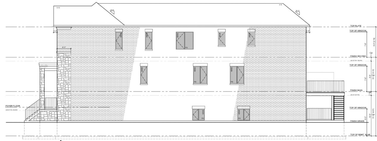
PROPOSED RIGHT SIDE ELEVATION SCALE AS NOTED OTHERWISE (UNIT 2)
