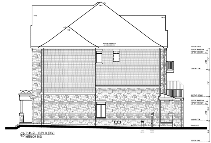
RIGHT SIDE ELEVATION - BLOCK 12
