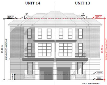
6 Unit 13-14 - Front Elevation - Height 1:100
