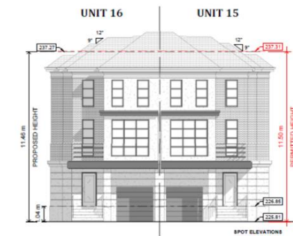
7 Unit 15-16 - Front Elevation - Height 1:100
