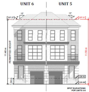
3 Unit 5-6 - Front Elevation - Height 1:100
