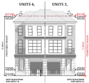
2 Unit 3, 4, 7, 8 - Front Elevation - Height 1:100
