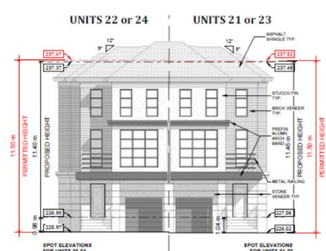
11 Unit 21-24 - Front Elevation - Height 1:100
