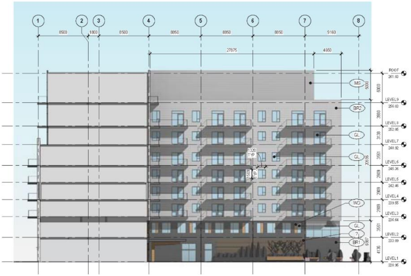
2 COURTYARD - SOUTH ELEVATION SCALE: 1:200
