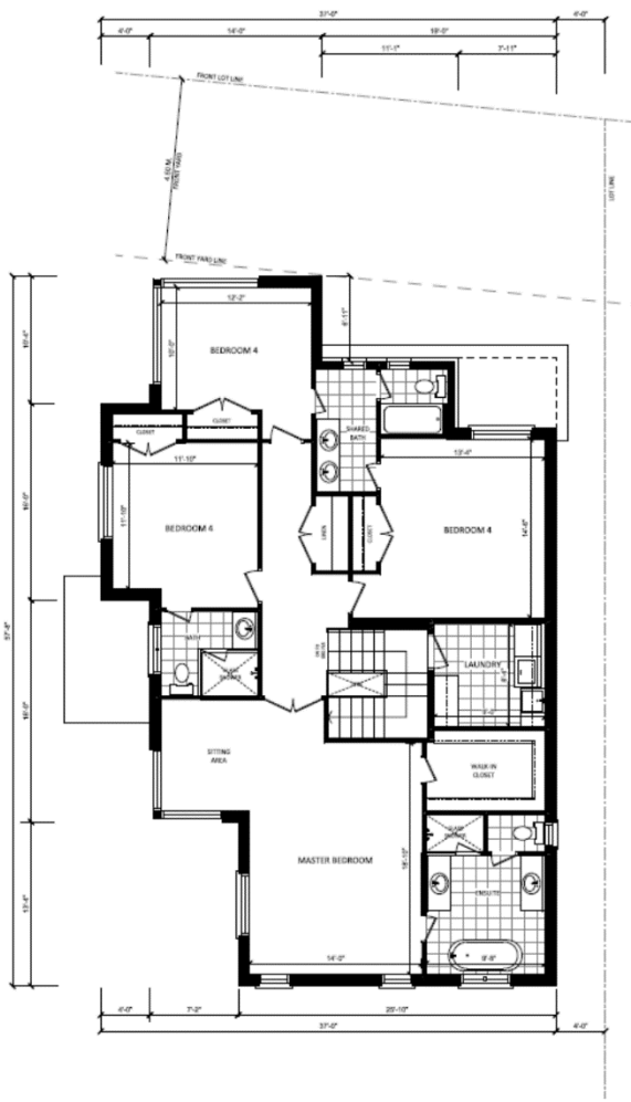
SECOND FLOOR PLAN (1,629 SQ. FT.)
