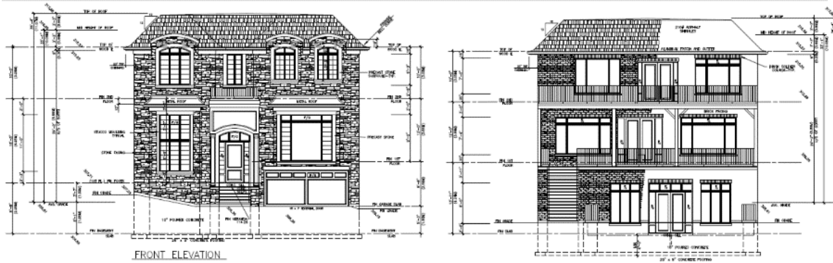
REAR ELEVATION
