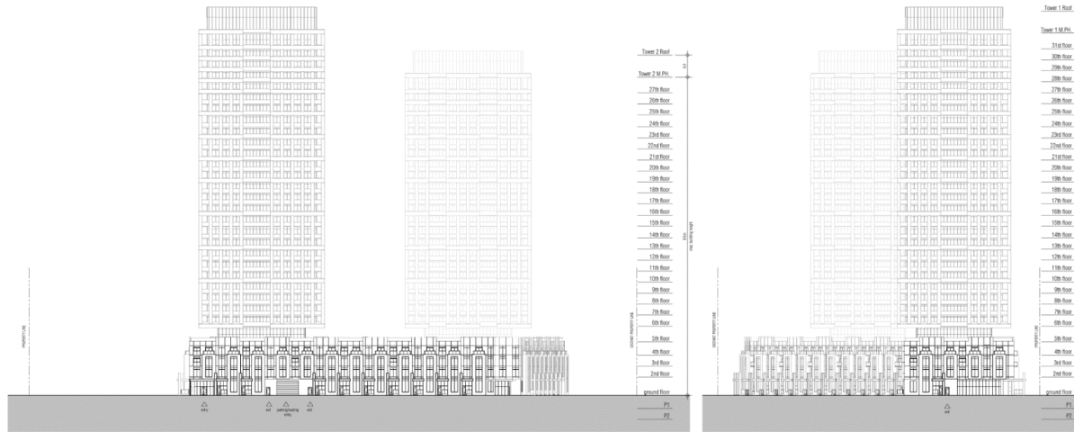
① West 1:400
