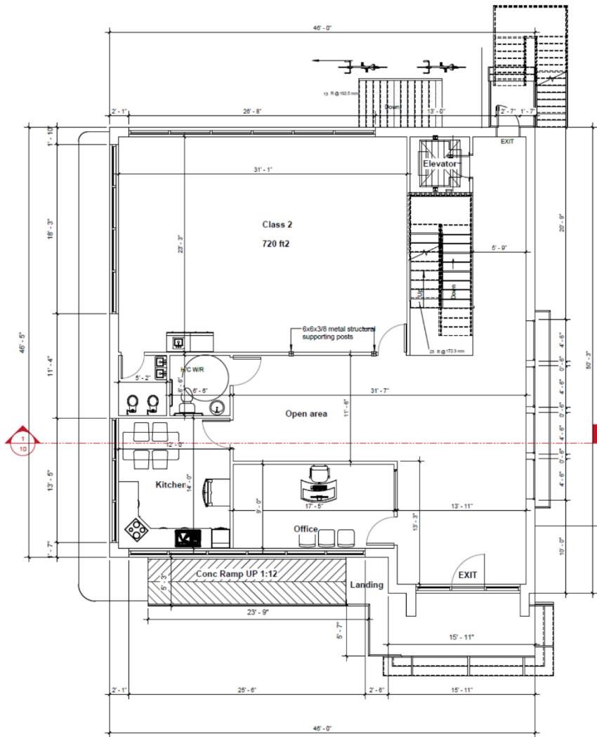
① First Floor 3/16" = 1'-0"
