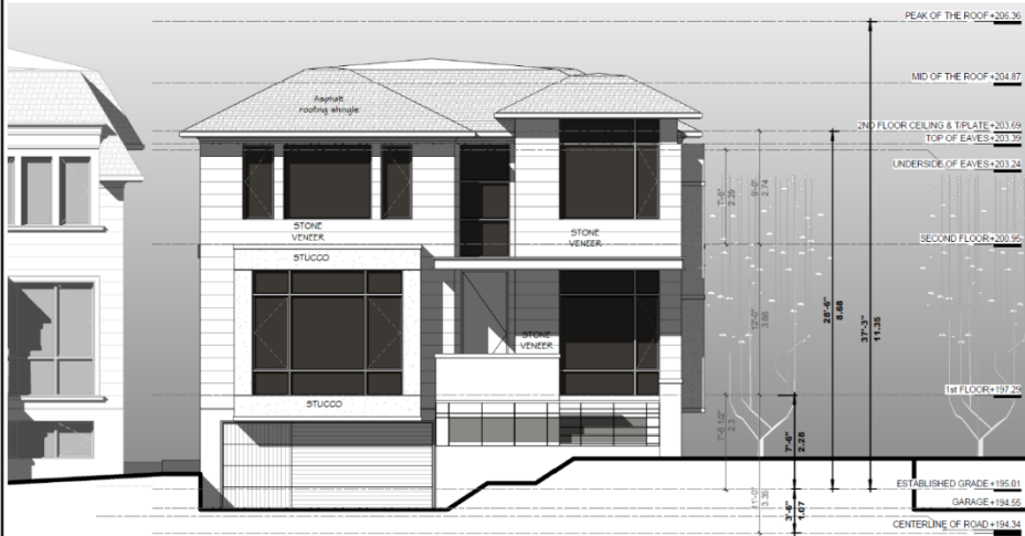
1 SOUTH ELEVATION PART A Scale: 1 : 75
