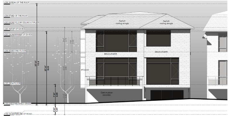
1 NORTH ELEVATION-PART A Scale: 1 : 75
