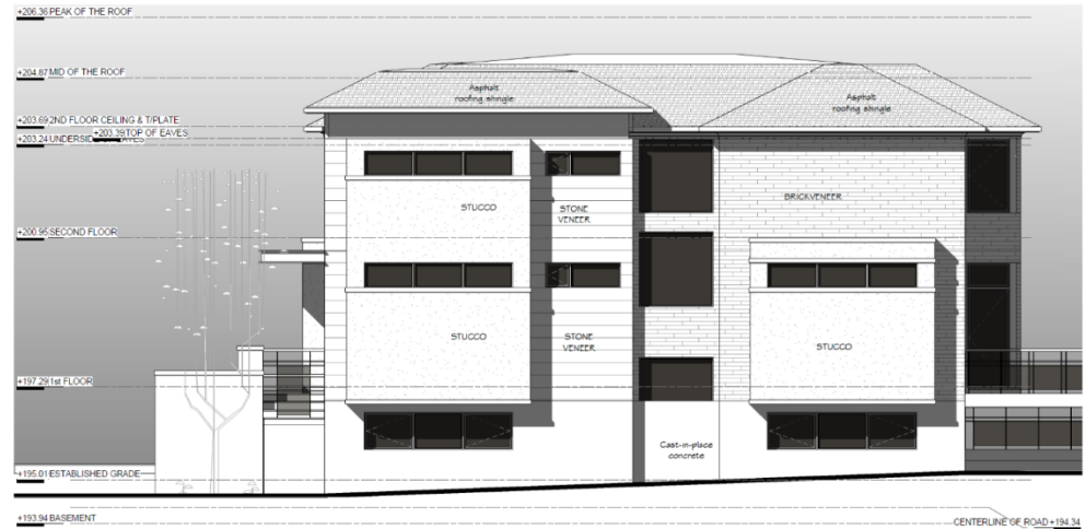
1 EAST ELEVATION-PART A Scale: 1 : 75
