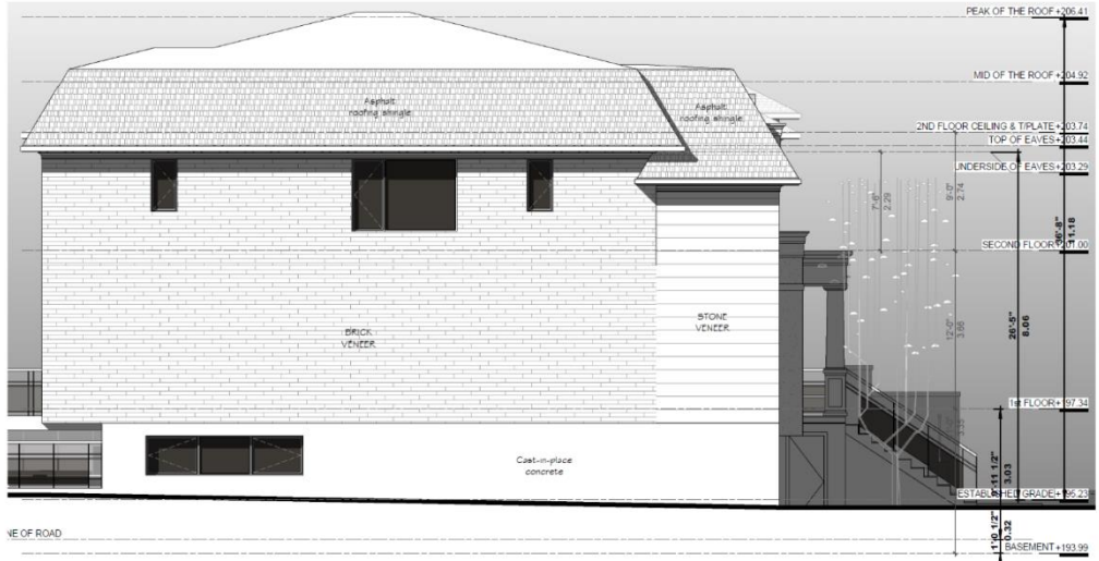
1 SOUTH ELEVATION PART B Scale: 1 : 75
