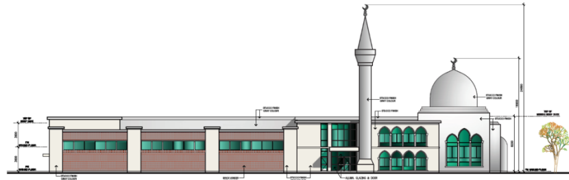
SOUTH ELEVATION (SCHOOL BLDG.) SCALE: 1:100
