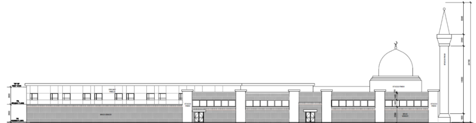
WEST ELEVATION (SCHOOL BLDG.) SCALE: 1:100
