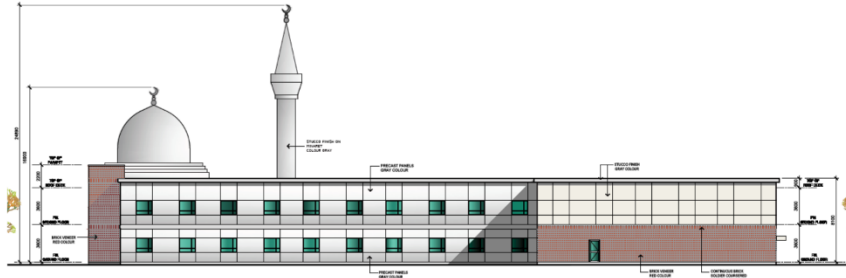
NORTH ELEVATION (SCHOOL BLDG.) SCALE: 1:100
