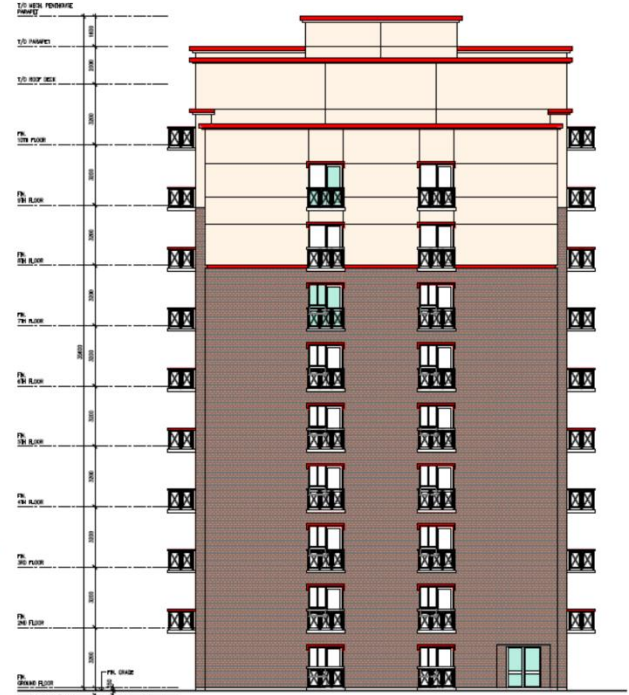
EAST ELEVATION (BLDG-C)
