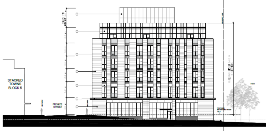
4 SOUTH ELEVATION - STREET 'A' Scale: 1:200
