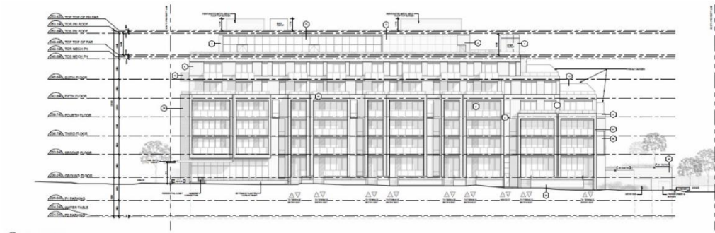
EAST ELEVATION
