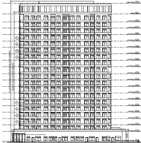
2 Building A - East Elevation
