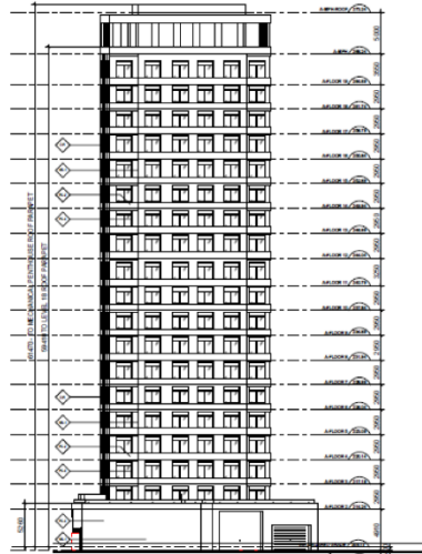
1 Building A - North Elevation
