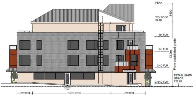
WEST ELEVATION
