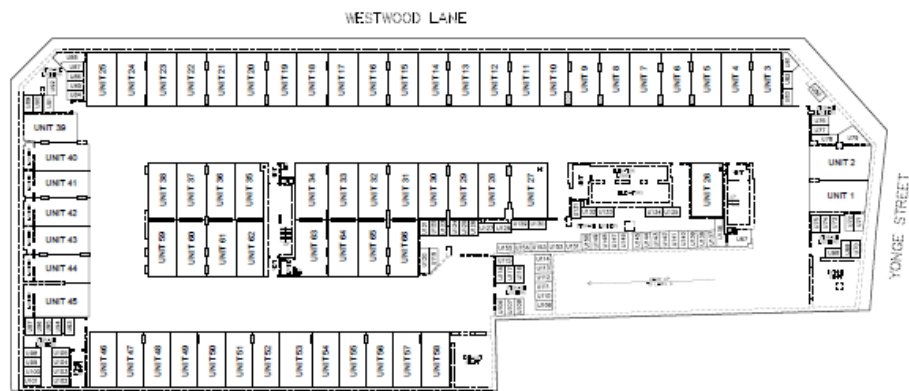
PLAN VIEW - ILLUSTRATIVE UNITS 1 TO 65 INCLUSIVE (Residential Parking) Includes 1 Accessible Parking and 7 Central Parking/Storage UNITS 67 TO 100 INCLUSIVE (Storage Locker) LEVEL B
