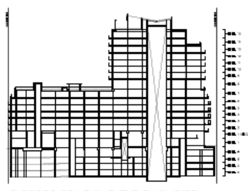
SCHEMATIC SECTION TO ILLUSTRATE RELATIONSHIP OF LEVELS
