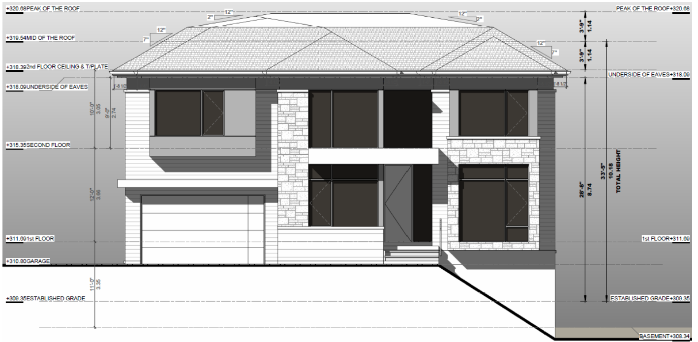
1 NORTH ELEVATION Scale: 1 : 75
