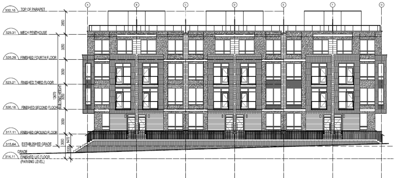
1 FRONT ELEVATION (BLOCK A) SCALE: 1:100
