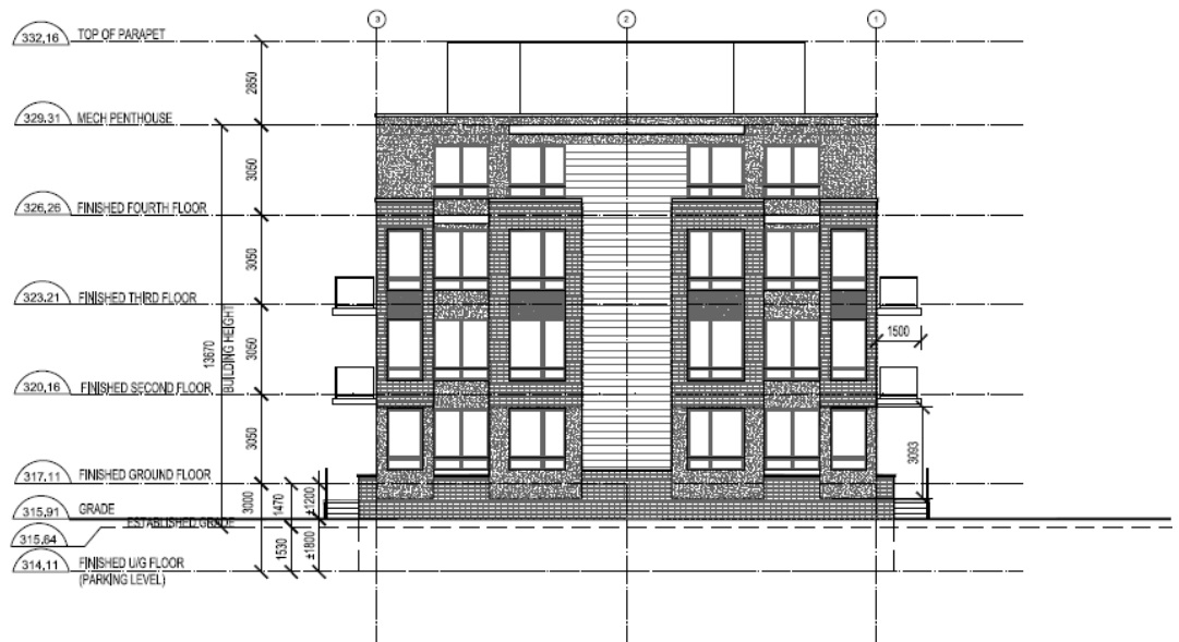
2 SIDE ELEVATION (BLOCK A) SCALE: 1:100
