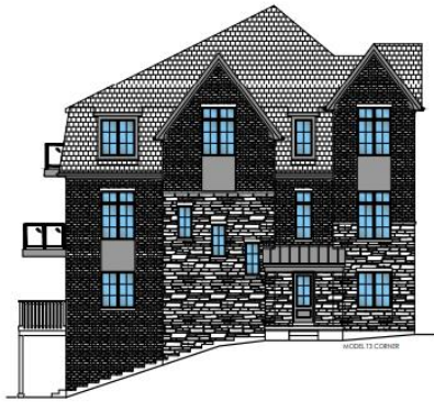
BLOCK A LEFT SIDE ELEVATION
