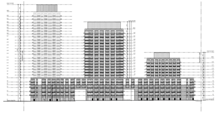
EAST ELEVATION SCALE 1/8"
