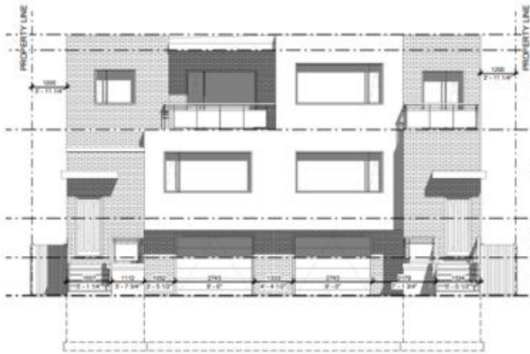
1 WEST ELEVATION 1 : 100
