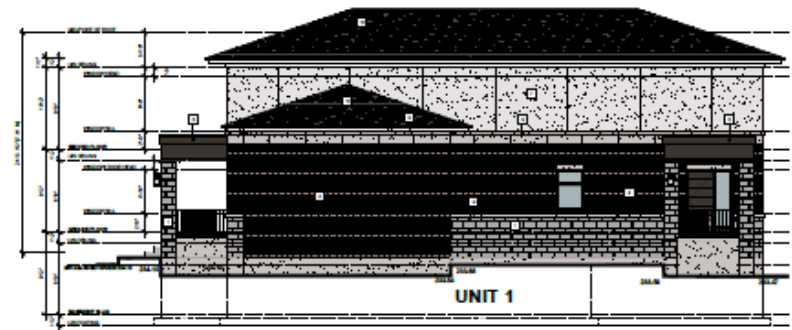
4 SOUTH ELEVATION A201/ 1/8" = 1'-0"
