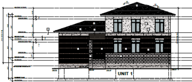
3 SOUTH ELEVATION A201/ 1/8" = 1'-0"
