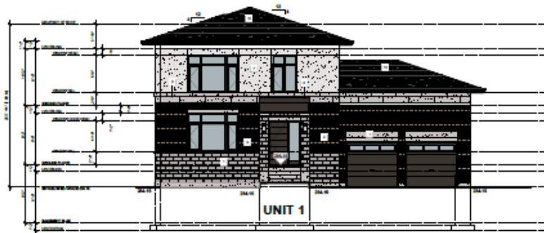
1 NORTH ELEVATION A201/ 1/8" = 1'-0"
