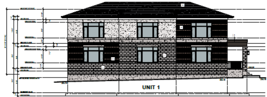
2 WEST ELEVATION A201/ 1/8" = 1'-0"
