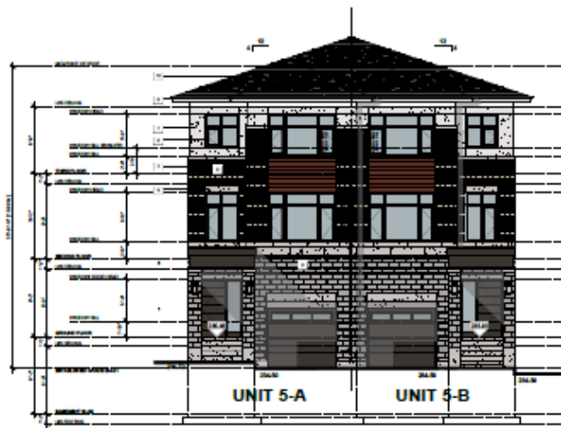
1 WEST ELEVATION A205 1/8"=1'-0"
