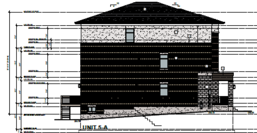
4 NORTH ELEVATION A205 1/8"=1'-0"
