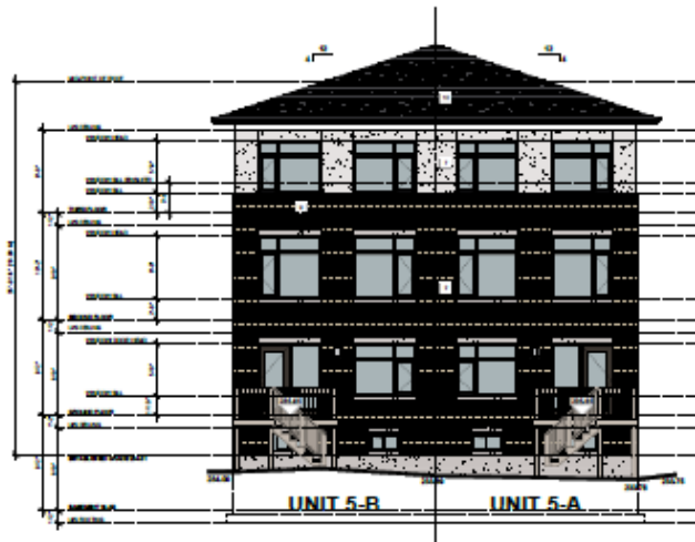
3 EAST ELEVATION A205 1/8"=1'-0"
