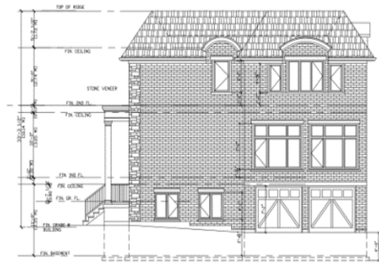
EAST ELEVATION
