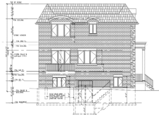
SIDE (WEST) ELEVATION
