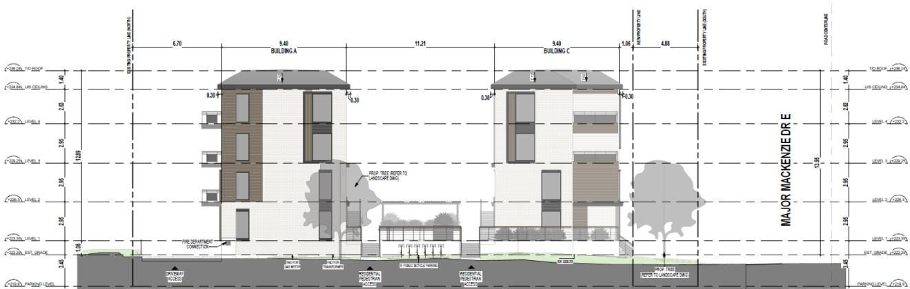
2 WEST ELEVATION AS 02 SCALE: 1:100
