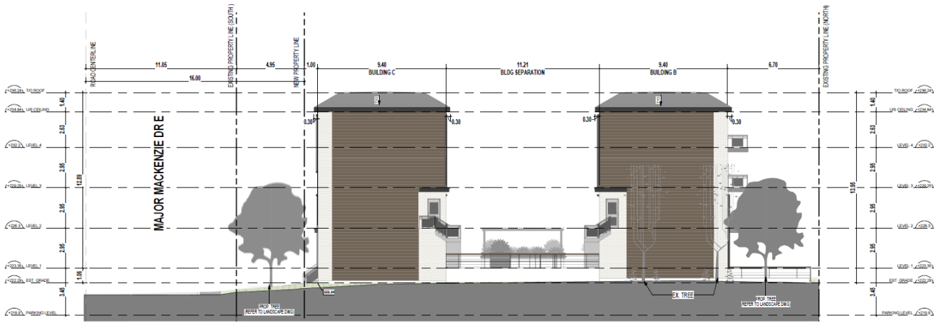
1 EAST ELEVATION AS 02 SCALE: 1:100
